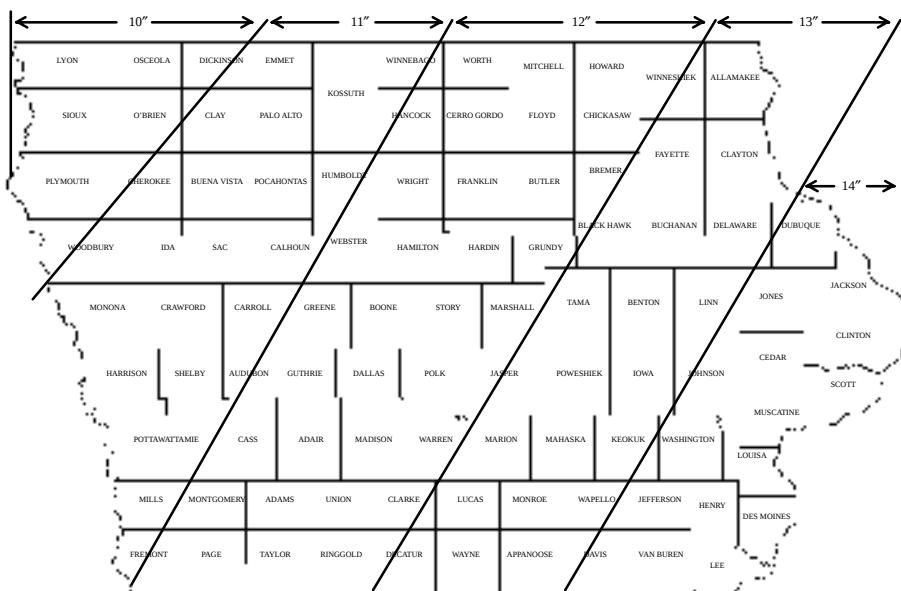
FIGURE 1. -- Feedlot runoff value, in inches, for determining required capacity of the “System 1: One Open Feedlot Effluent Application Period Per Year” manure control system.
