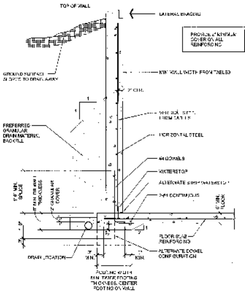
APPENDIX D, FIGURE D-1 MONOLITHIC FOOTING FLOOR DETAIL
