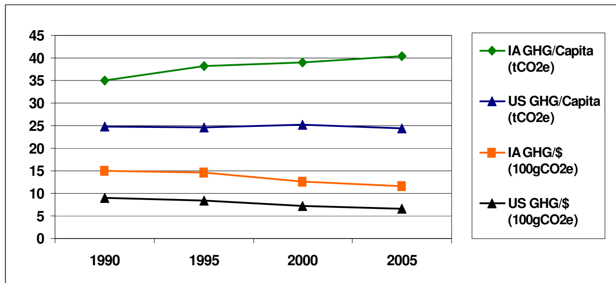
Figure 2-1. Iowa and U.S. gross GHG emissions, per-capita and per-unit gross product
