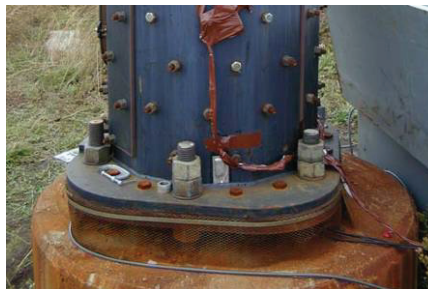
Bolted Reinforcing Jacket
