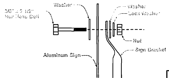
SIGN INSTALLATION DETAIL
