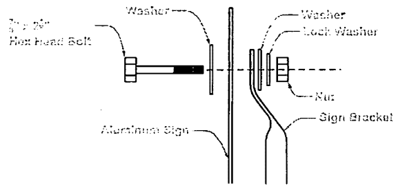
SIGN INSTALLATION DETAIL
