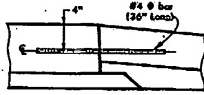
DETAIL B NON-REINFORCED P.C. CONCRETE PAVEMENT
