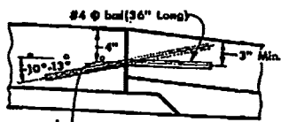
DETAIL A CONTINUOUSLY REINFORCED P.C. CONCRETE PAVEMENT
