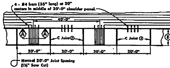
TYPICAL PLAN P.C. CONCRETE REINFORCED P.C. CONCRETE PAVEMENT ADJACENT TO CONTINUOUSLY REINFORCED P.C. CONCRETE PAVEMENT
