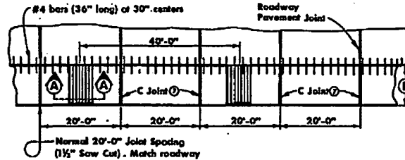
TYPICAL PLAN P.C. CONCRETE PAVED SHOULDERS ADJACENT TO NON-REINFORCED P.C. CONCRETE PAVEMENT
