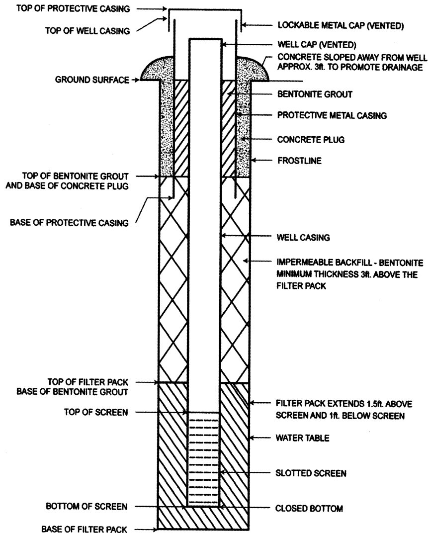
Figure 1 Typical Monitoring Well Cross Section
